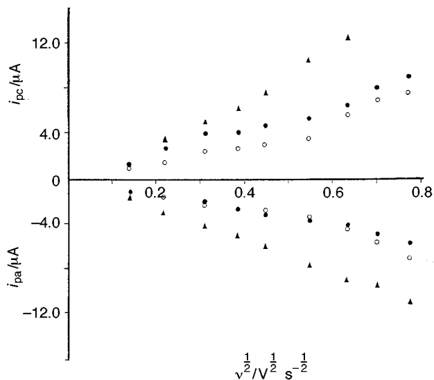
Fig. 3 Plots of i pc and i pa vs. the square root of the scan rate for 10 -3 M hemin at pH 8.0 (buffer 0.05 M Tris) encapsulated in sds (○), Triton X-100 (●) and NMe 3 (C 16 H 33 )Br (▲) micelles
