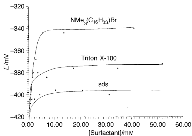
Fig. 1 Change of E_2 with surfactant concentration ( 10^{-3} M hemin at pH 8.0, 0.05 M Tris buffer) †
